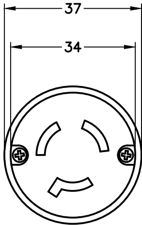
NEMA L6-15 CONNECTOR FRONT VIEW
